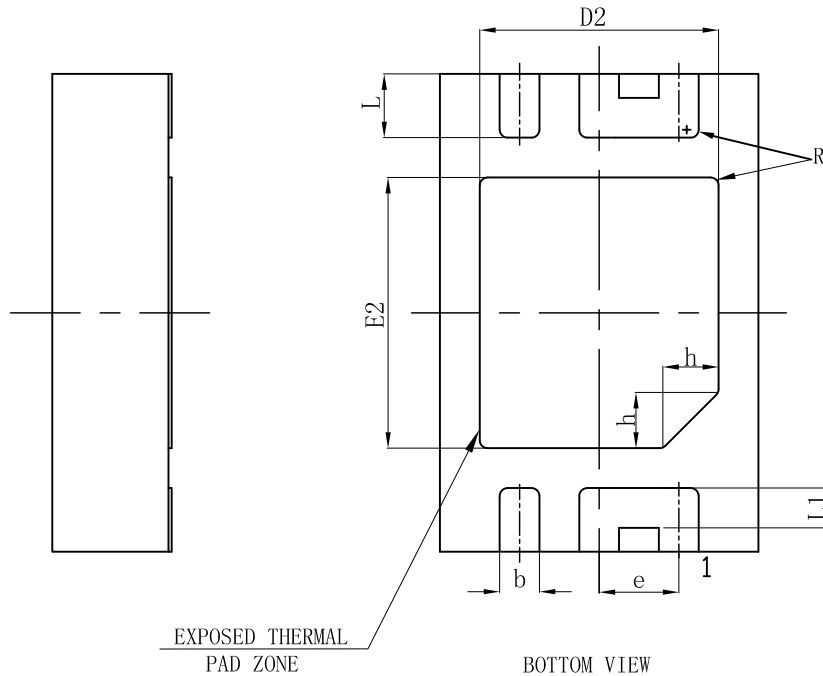
BOTTOM VIEW
