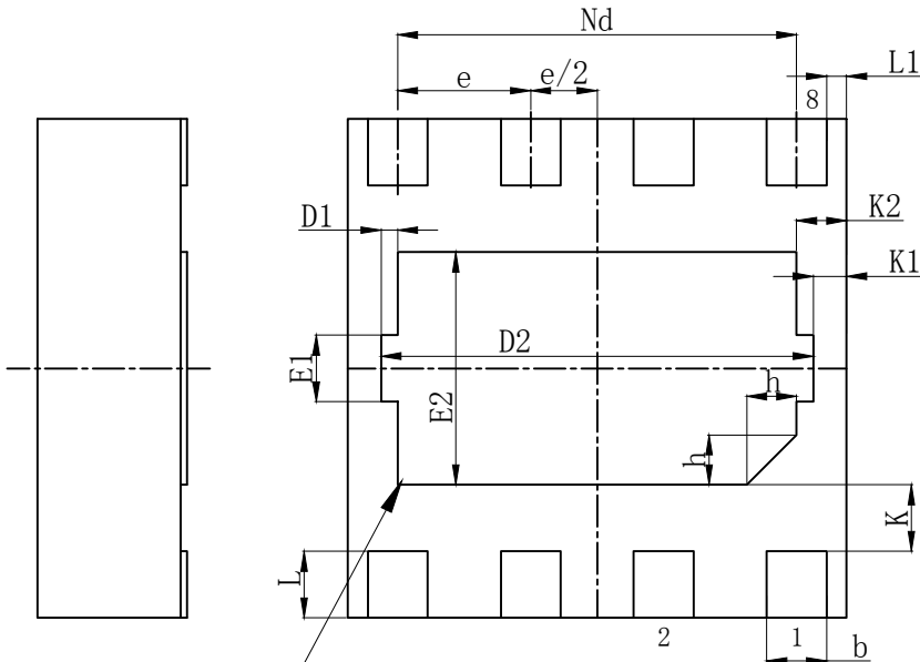
BOTTOM VIEW
