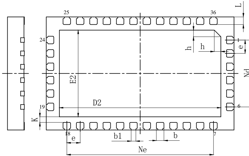
BOTTOM VIEW
