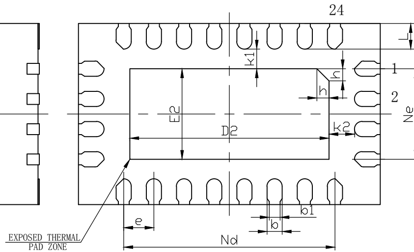
BOTTOM VIEW
