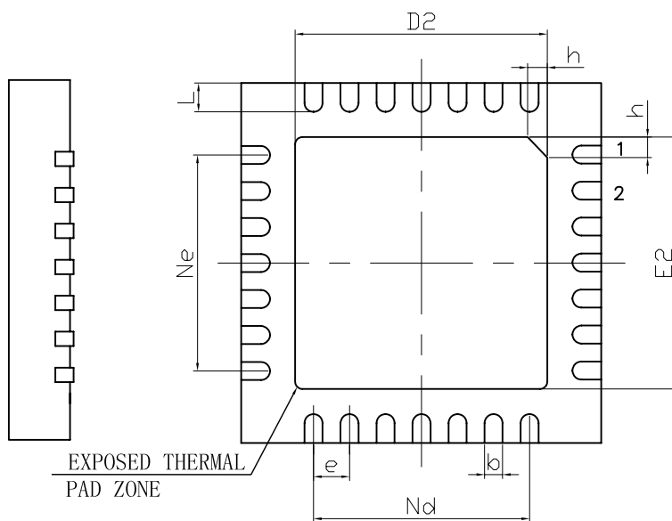
BOTTOM VIEW
