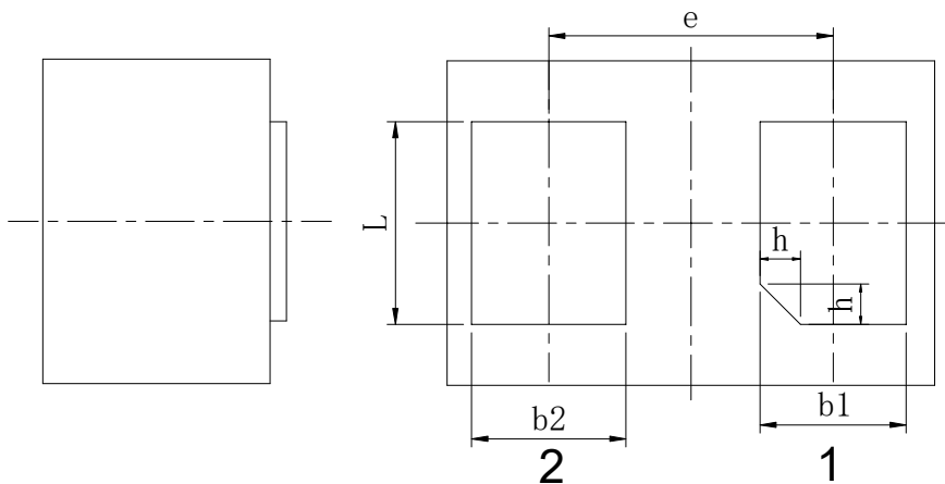
BOTTOM VIEW
